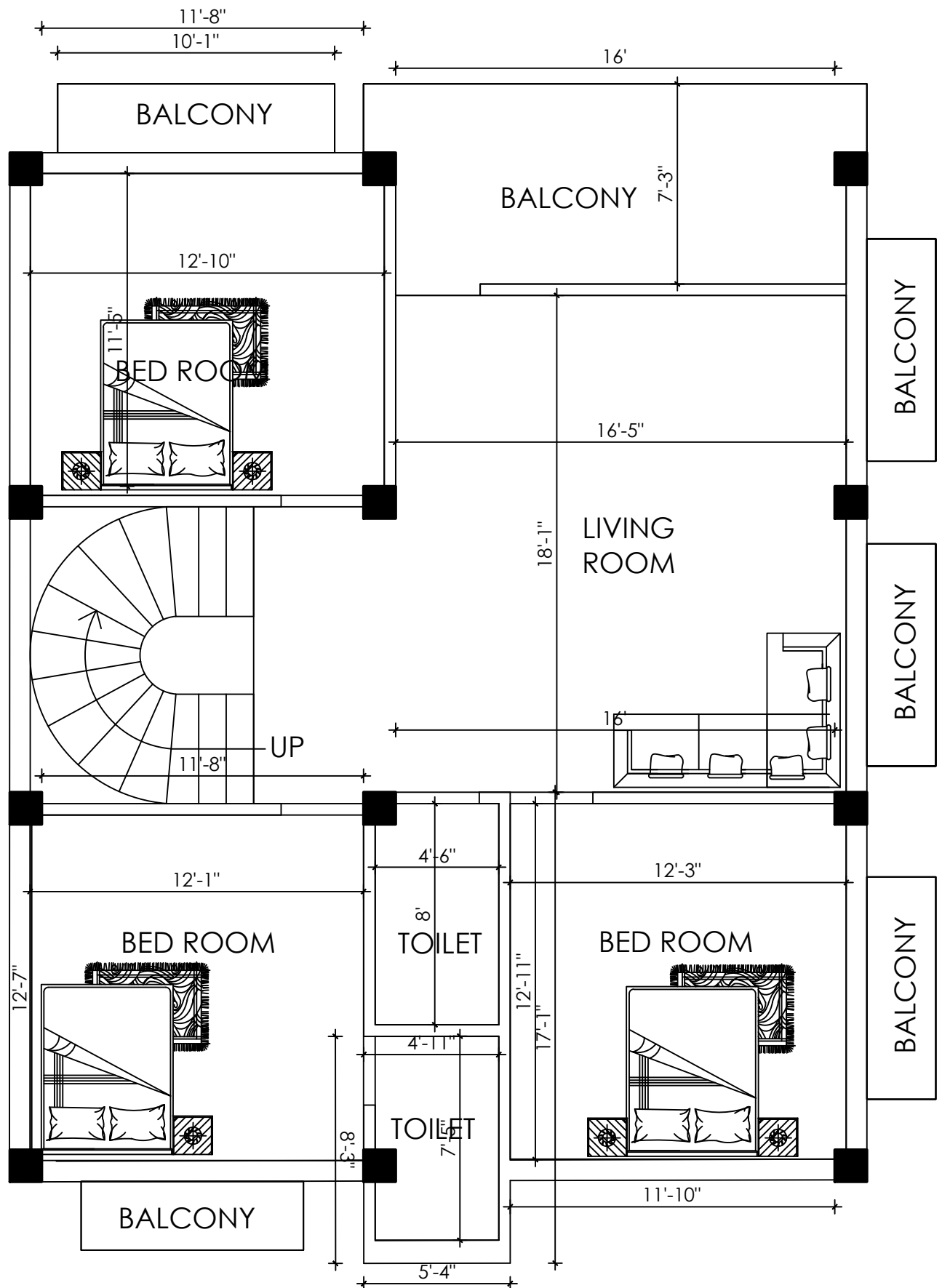
SECOND FLOOR PLAN AREA = 1100 SQ.FT
